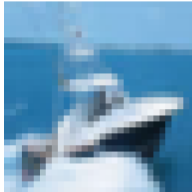
Ship
